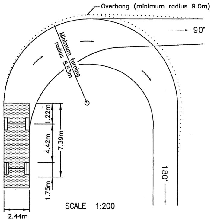
TRACKING CURVE FOR 90 PERCENTILE TRUCK
