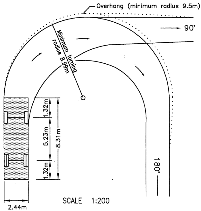
TRACKING CURVE FOR 99 PERCENTILE TRUCK
