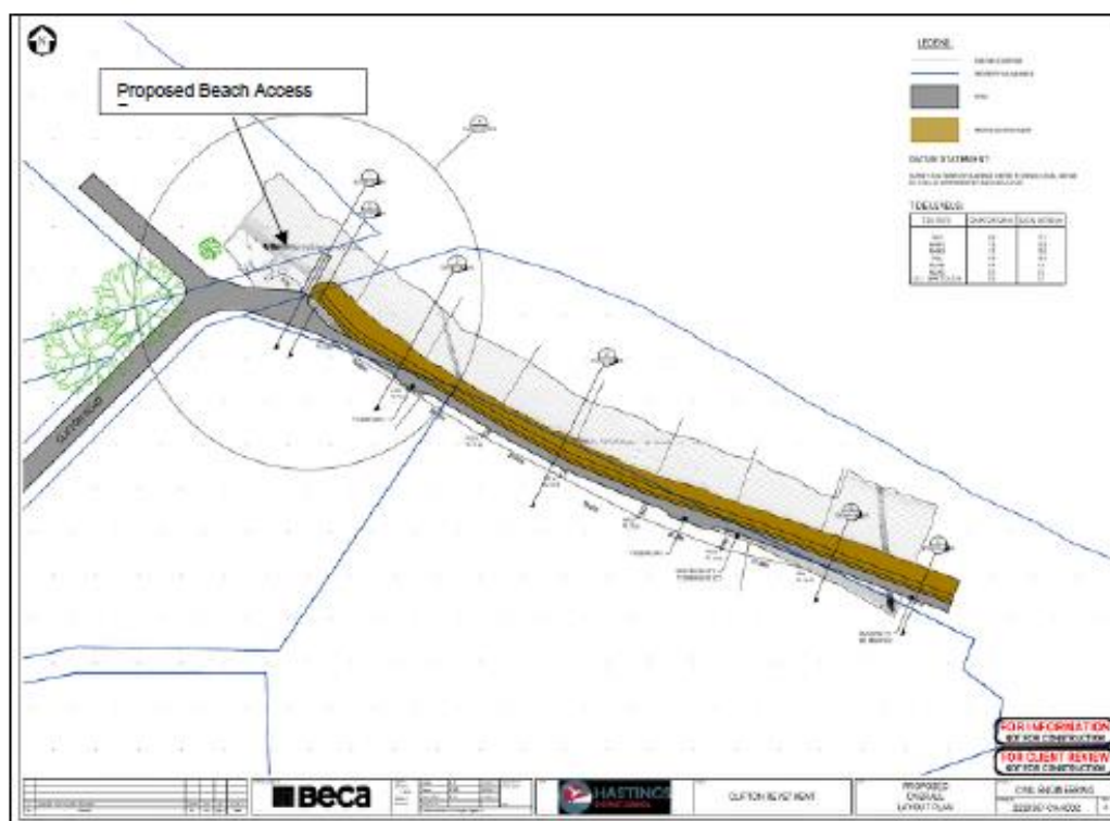
Figure 3: Proposed Revetment 1
